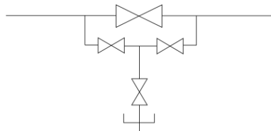
Principal scheme
